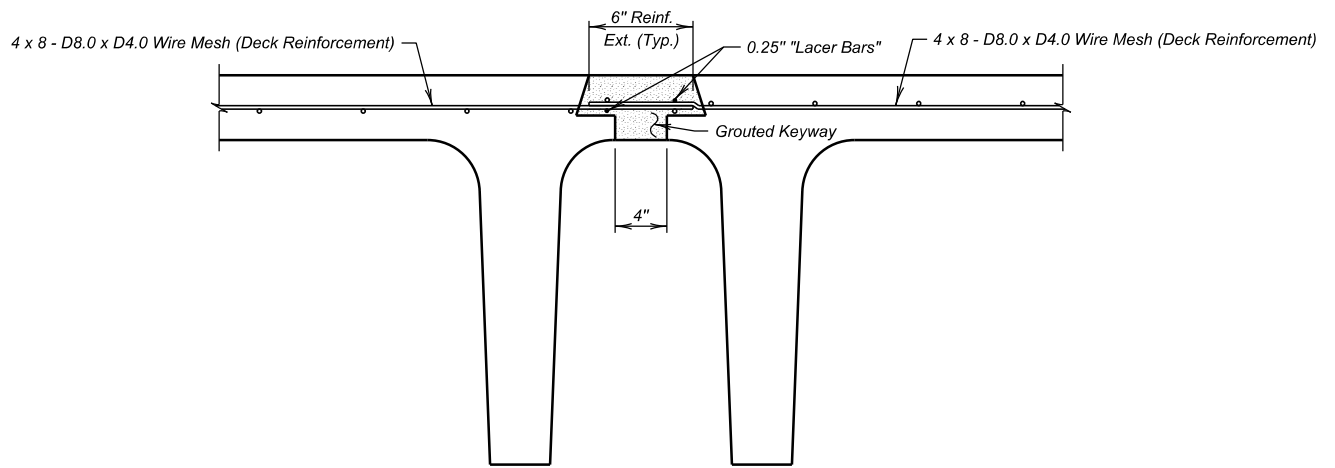
DOUBLE TEE LONGITUDINAL JOINT DETAIL
